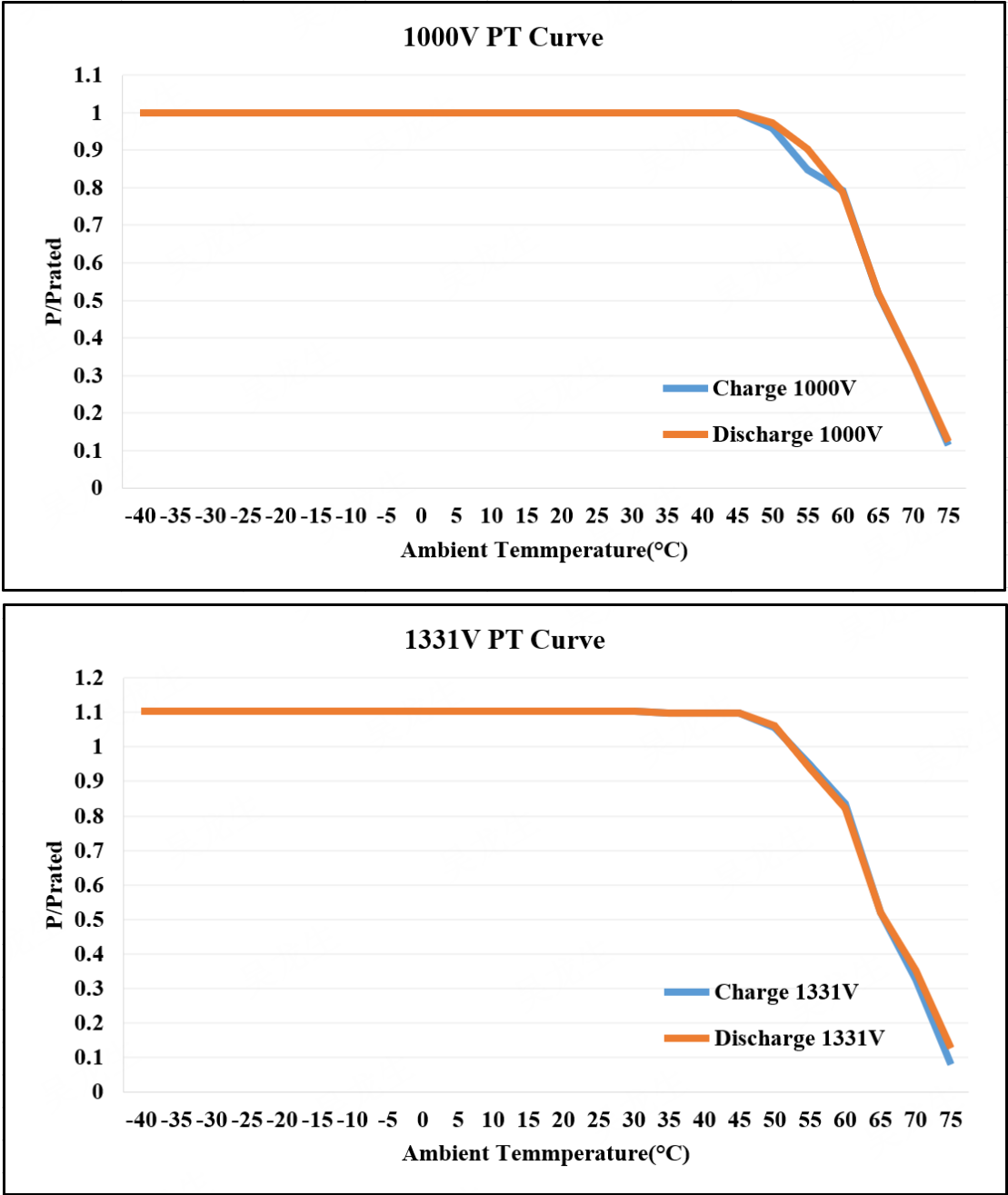
Temperature Derating Curve
