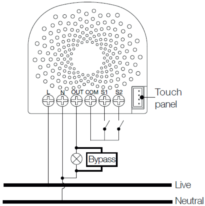
3-wire connection with neutral and bypass load.
