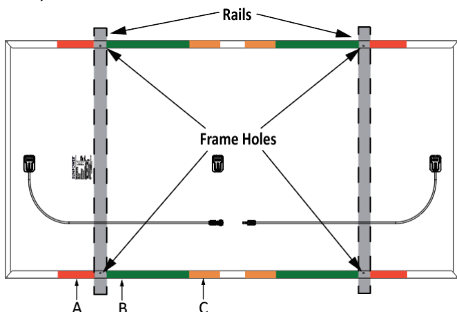
Figure 4: Mounting Zone Locations for Performance modules
